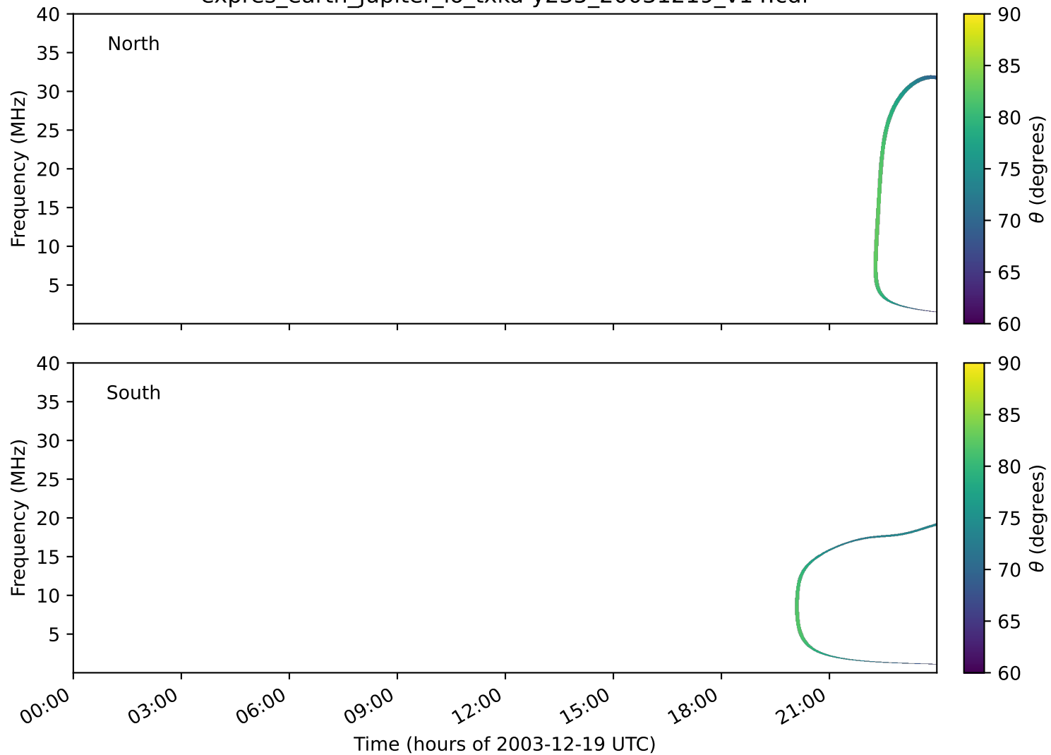
expres_earth_jupiter_io_txka-y235_20031219_v14.cdf
