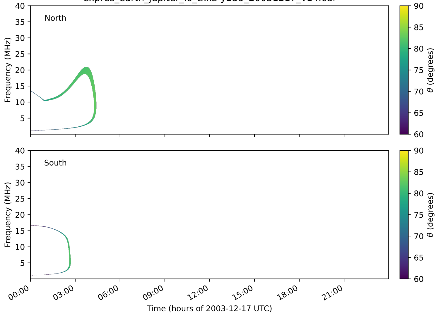
expres_earth_jupiter_io_txka-y235_20031217_v14.cdf
