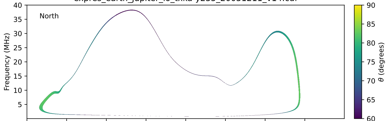
expres_earth_jupiter_io_txka-y235_20031211_v14.cdf
