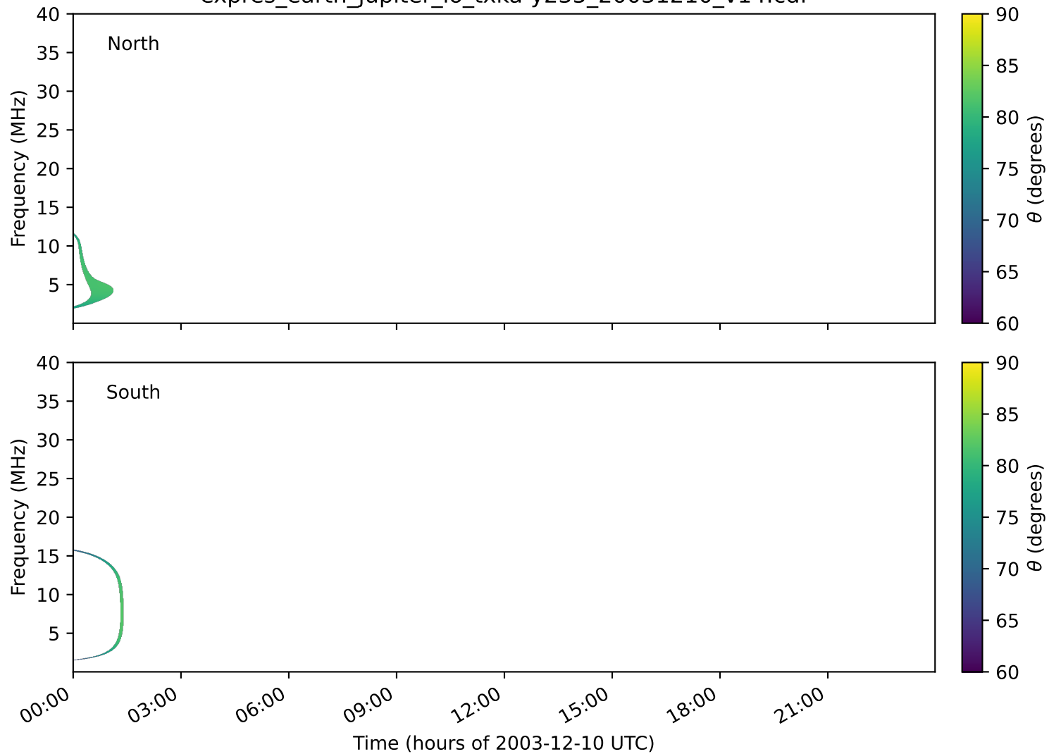
expres_earth_jupiter_io_txka-y235_20031210_v14.cdf
