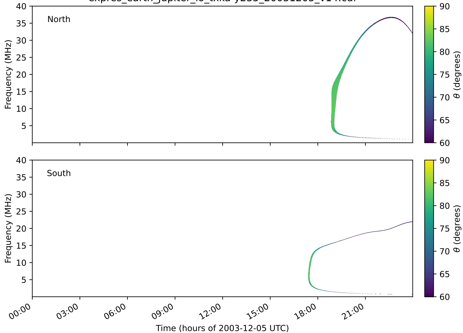
expres_earth_jupiter_io_txka-y235_20031205_v14.cdf
