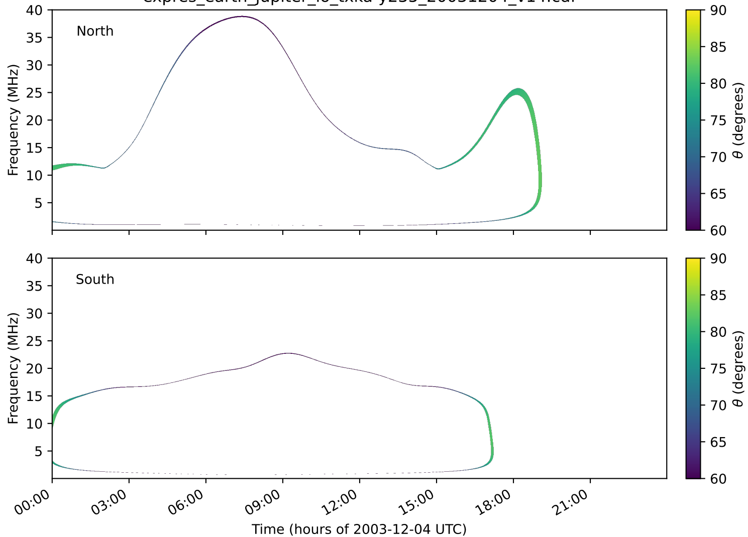
expres_earth_jupiter_io_txka-y235_20031204_v14.cdf
