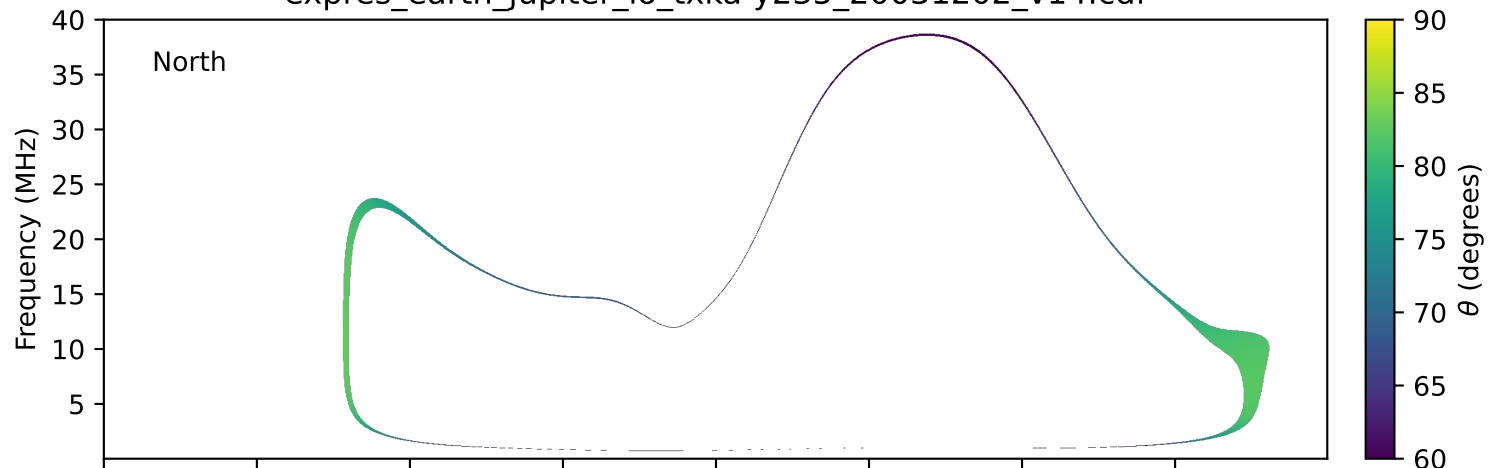
expres_earth_jupiter_io_txka-y235_20031202_v14.cdf
