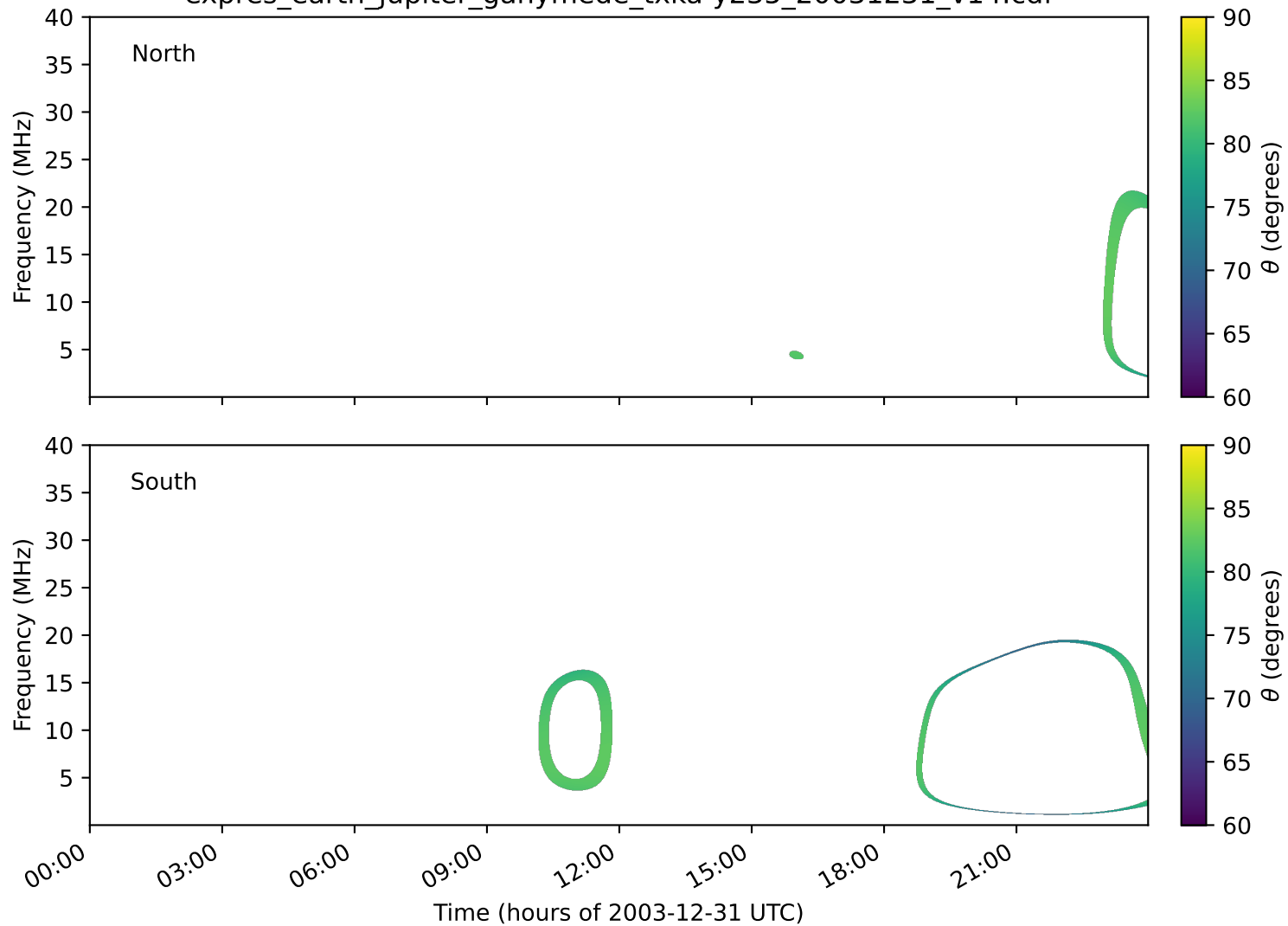
expres_earth_jupiter_ganymede_txka-y235_20031231_v14.cdf
