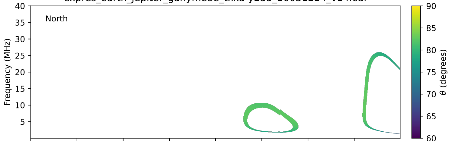
expres_earth_jupiter_ganymede_txka-y235_20031224_v14.cdf
