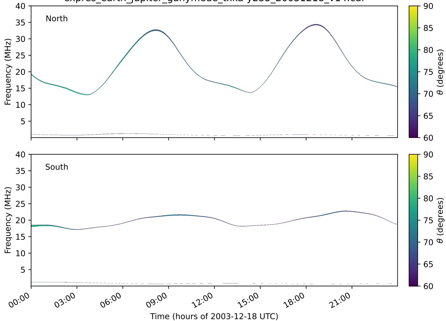
expres_earth_jupiter_ganymede_txka-y235_20031218_v14.cdf
