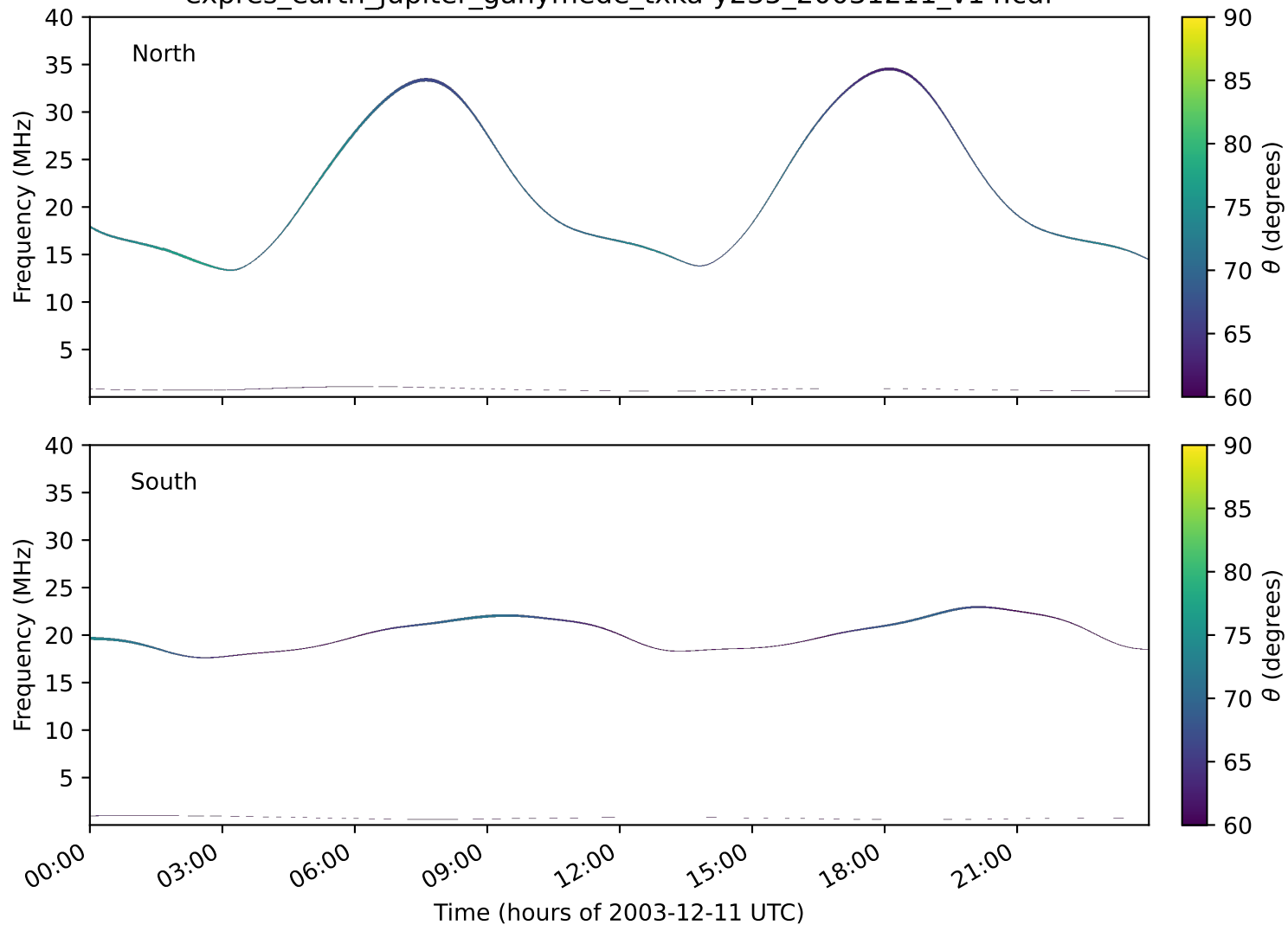
expres_earth_jupiter_ganymede_txka-y235_20031211_v14.cdf
