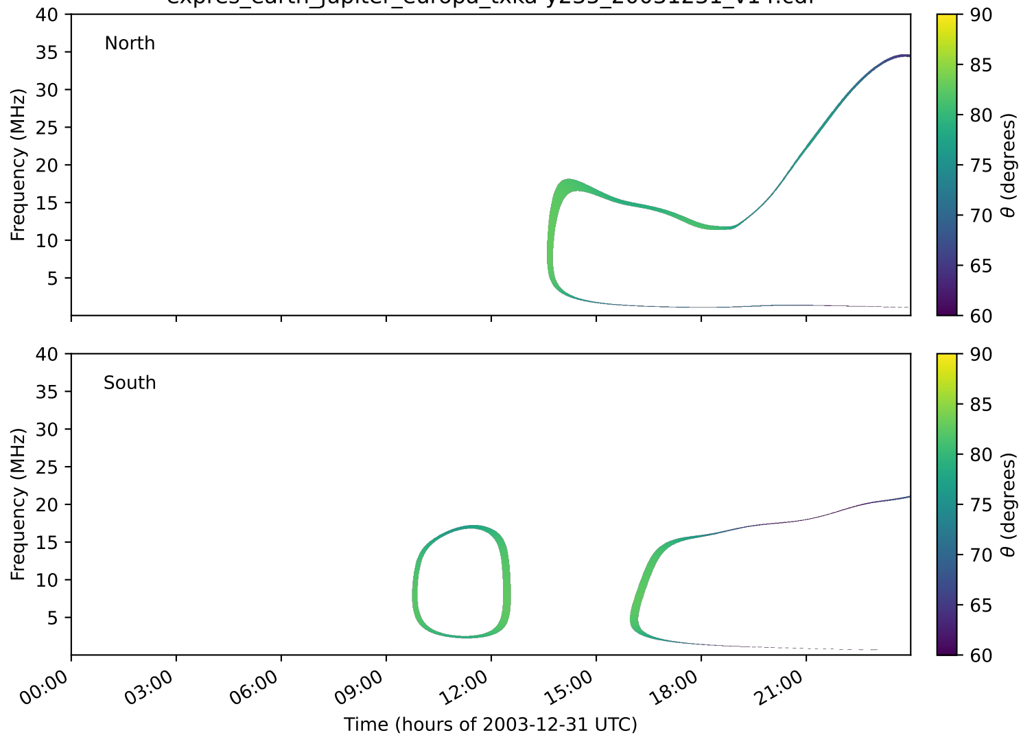
expres_earth_jupiter_europa_txka-y235_20031231_v14.cdf
