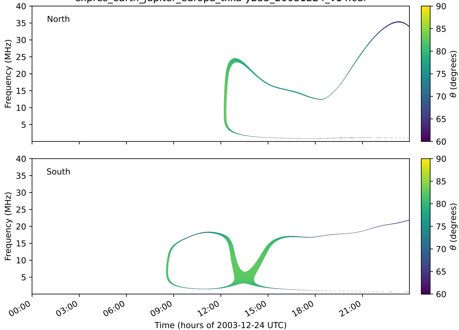
expres_earth_jupiter_europa_txka-y235_20031224_v14.cdf
