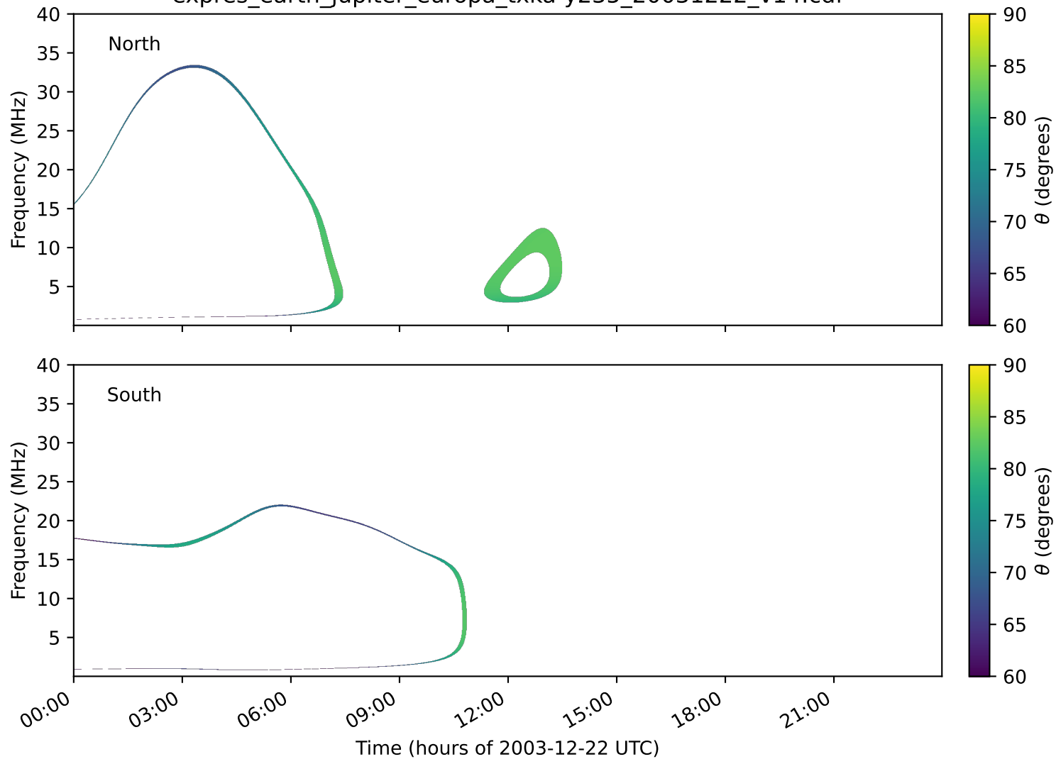
expres_earth_jupiter_europa_txka-y235_20031222_v14.cdf
