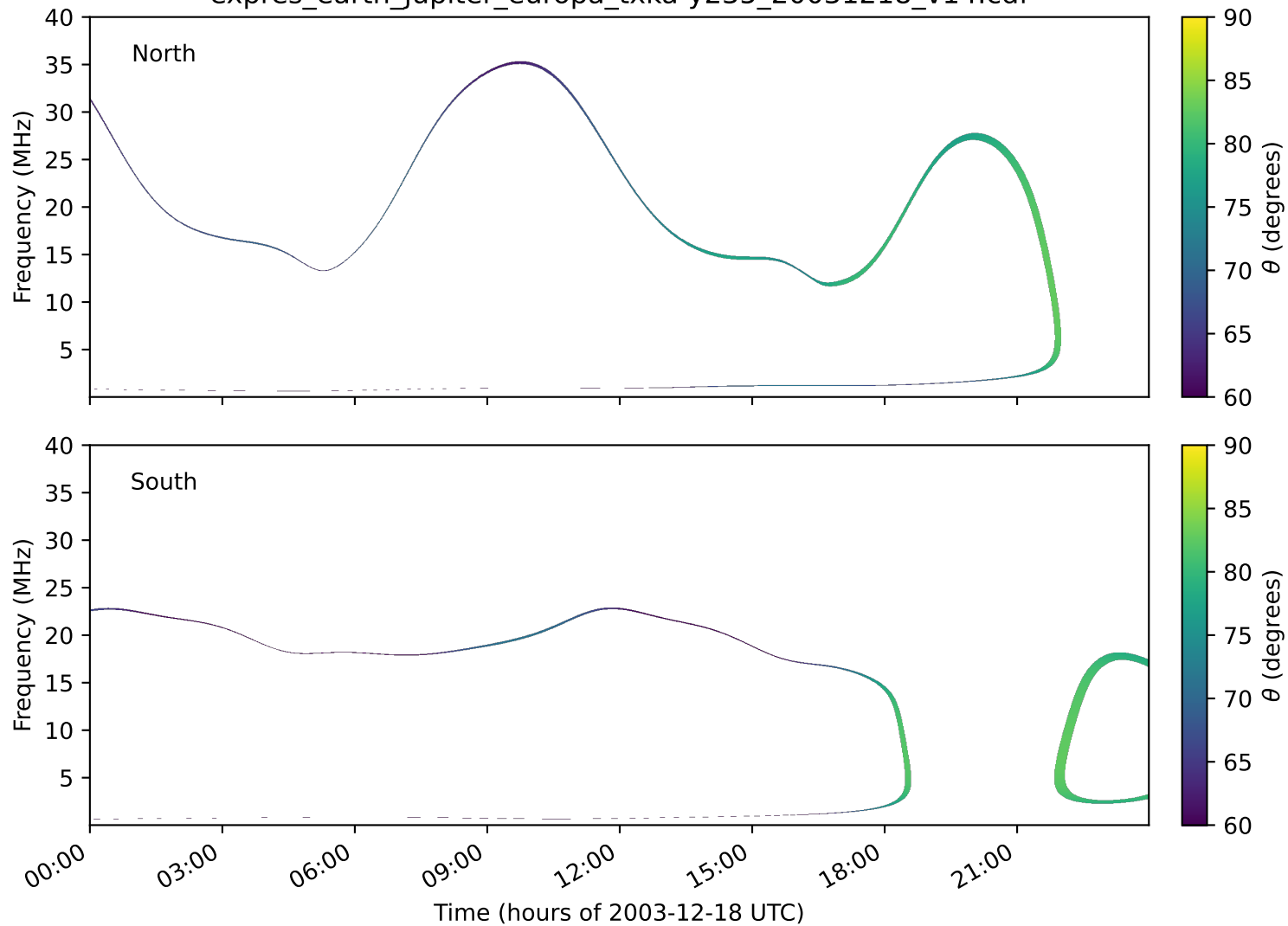
expres_earth_jupiter_europa_txka-y235_20031218_v14.cdf
