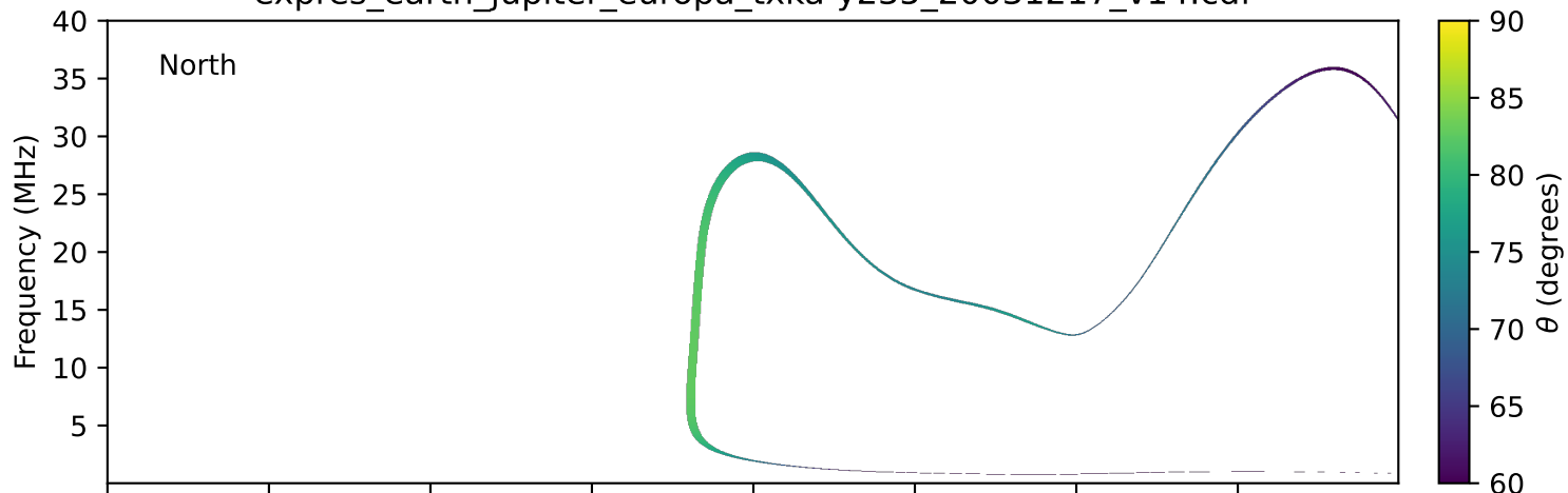
expres_earth_jupiter_europa_txka-y235_20031217_v14.cdf
