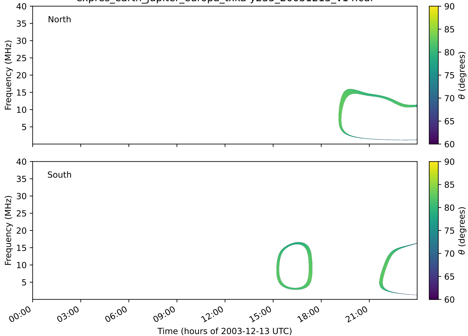
expres_earth_jupiter_europa_txka-y235_20031213_v14.cdf
