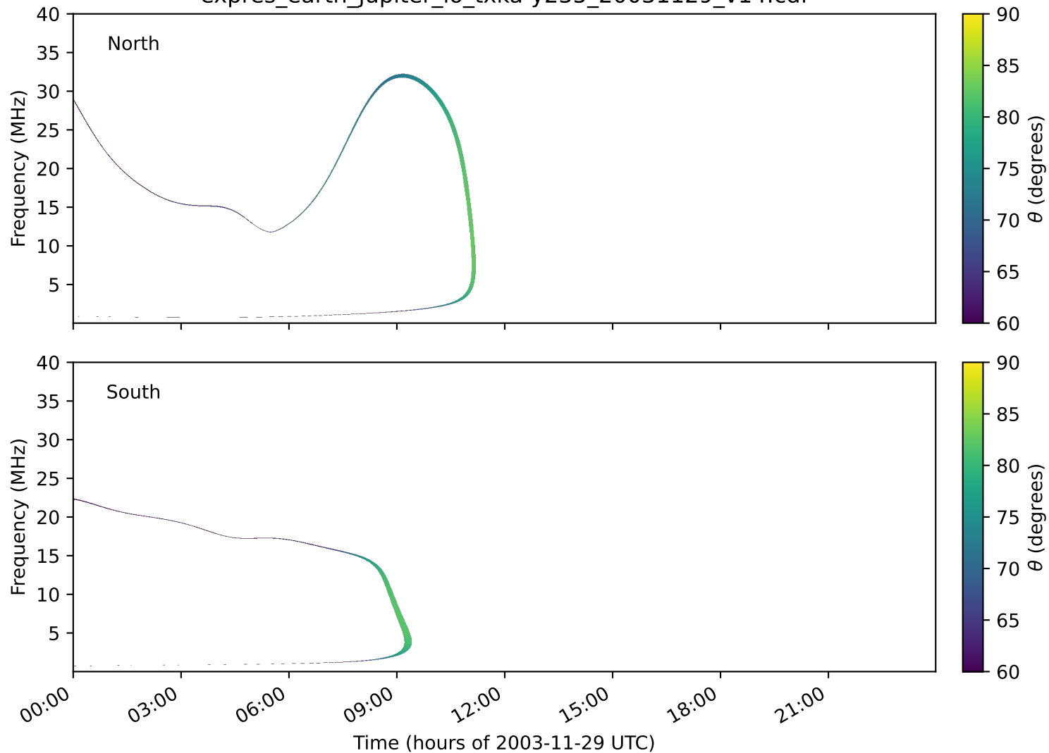
expres_earth_jupiter_io_txka-y235_20031129_v14.cdf
