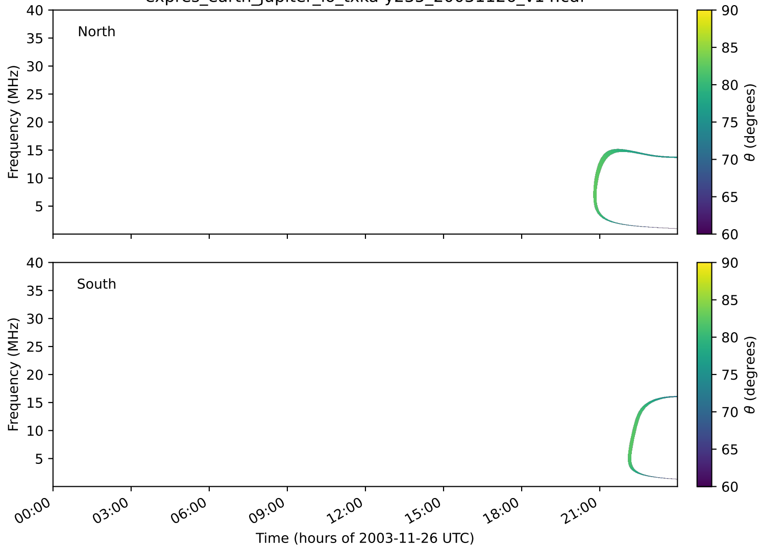
expres_earth_jupiter_io_txka-y235_20031126_v14.cdf
