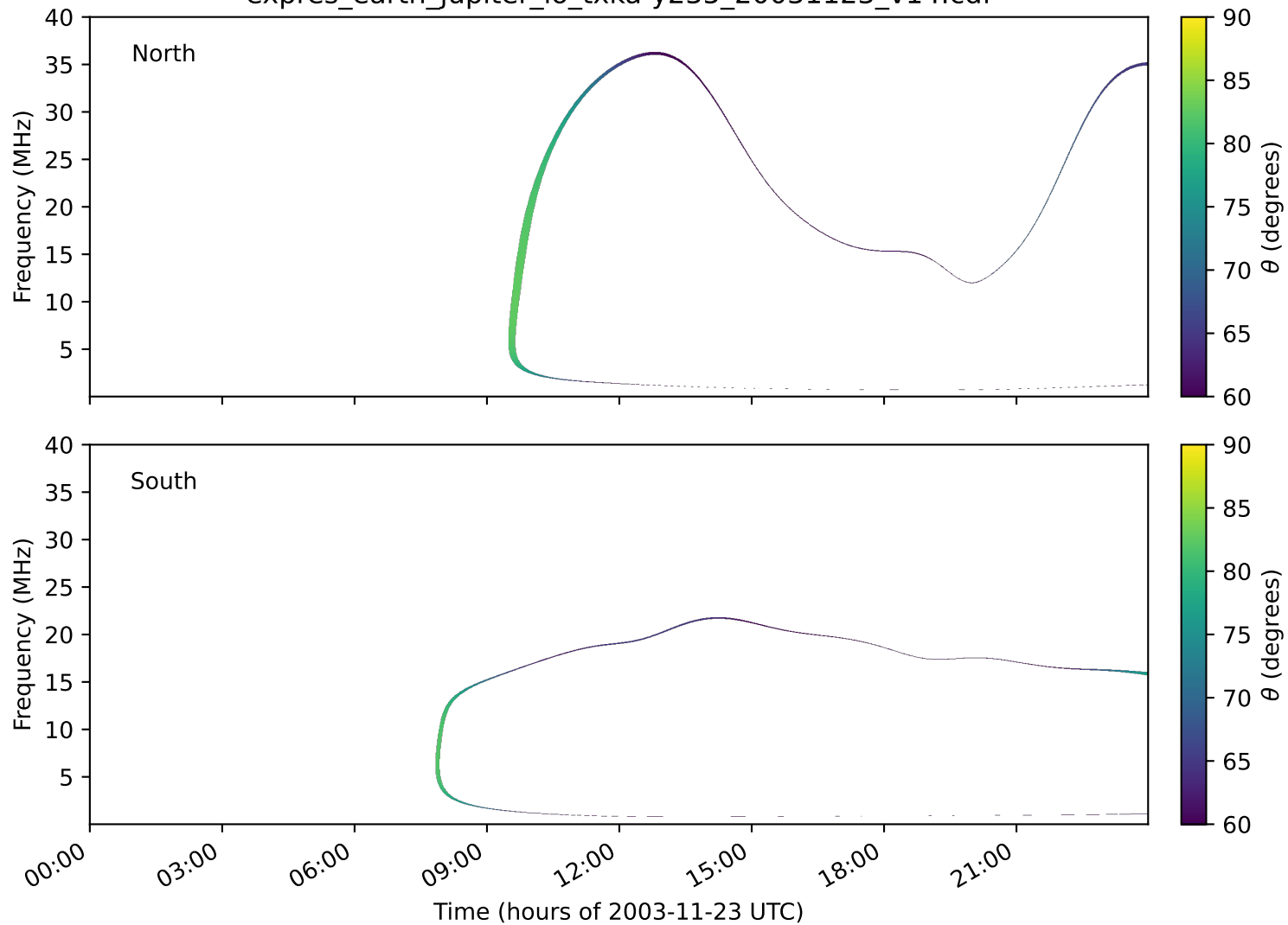
expres_earth_jupiter_io_txka-y235_20031123_v14.cdf
