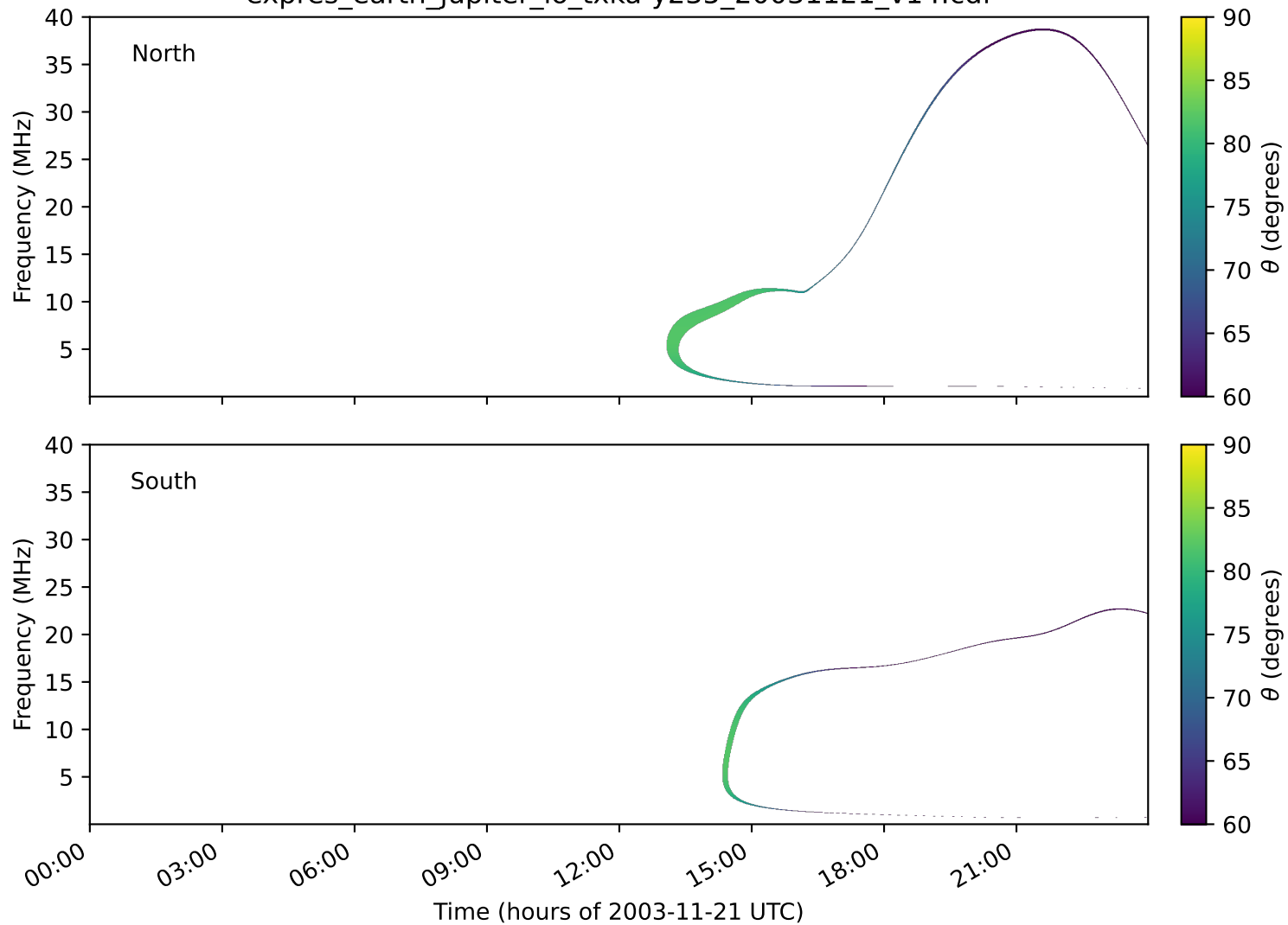
expres_earth_jupiter_io_txka-y235_20031121_v14.cdf
