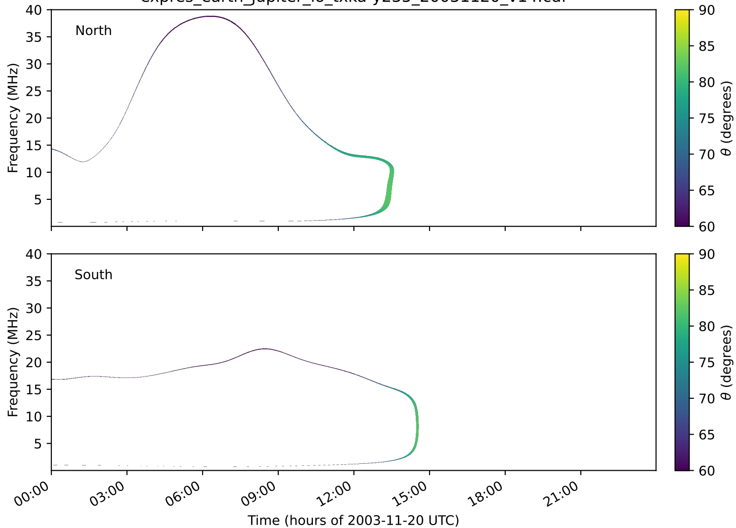
expres_earth_jupiter_io_txka-y235_20031120_v14.cdf
