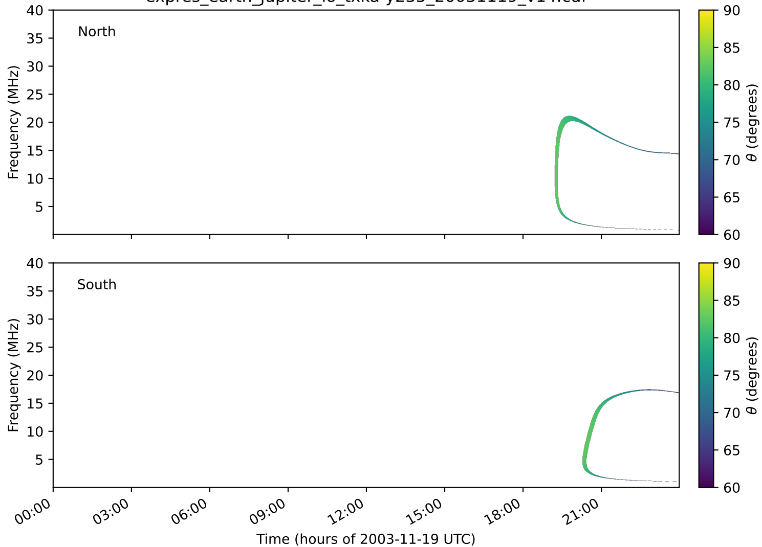
expres_earth_jupiter_io_txka-y235_20031119_v14.cdf
