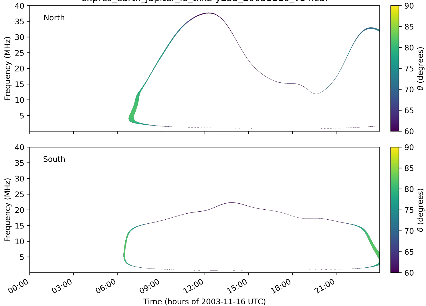
expres_earth_jupiter_io_txka-y235_20031116_v14.cdf
