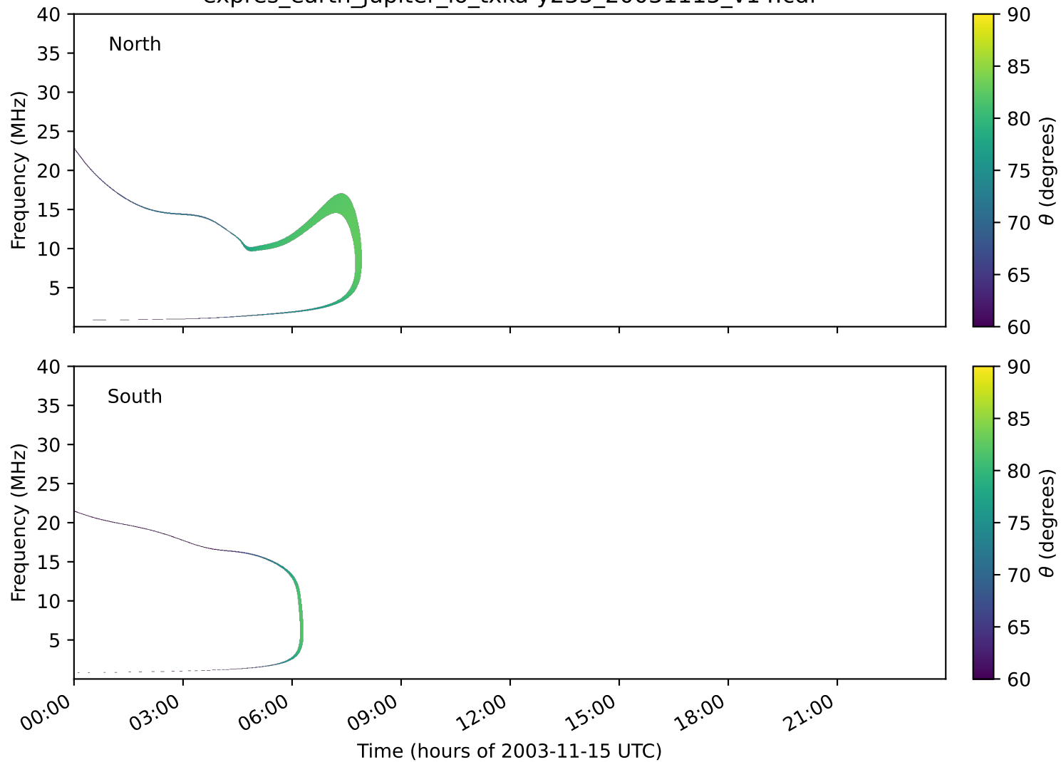
expres_earth_jupiter_io_txka-y235_20031115_v14.cdf
