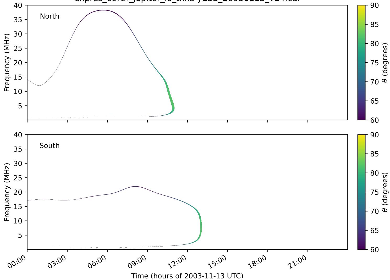
expres_earth_jupiter_io_txka-y235_20031113_v14.cdf
