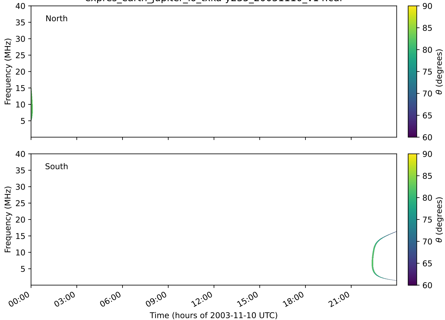
expres_earth_jupiter_io_txka-y235_20031110_v14.cdf
