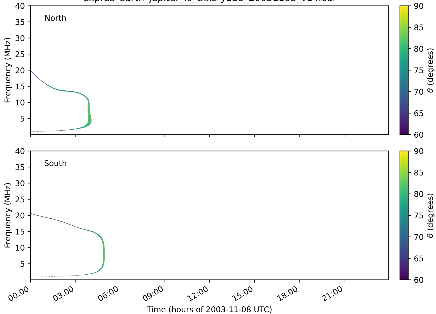
expres_earth_jupiter_io_txka-y235_20031108_v14.cdf
