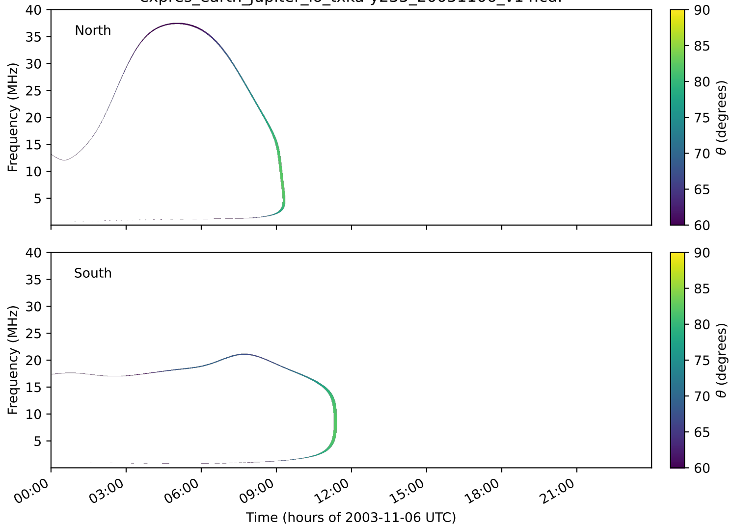
expres_earth_jupiter_io_txka-y235_20031106_v14.cdf
