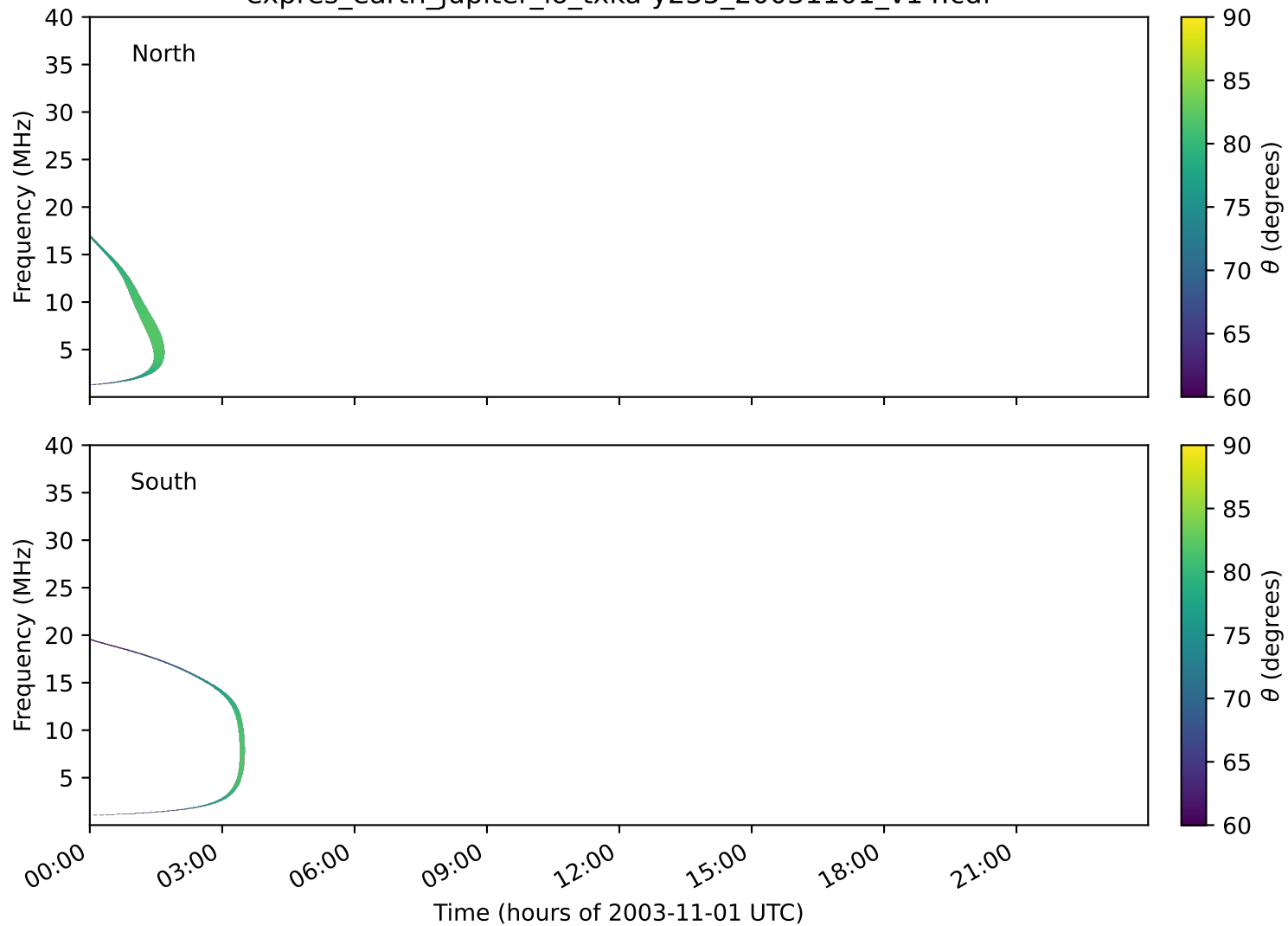
expres_earth_jupiter_io_txka-y235_20031101_v14.cdf
