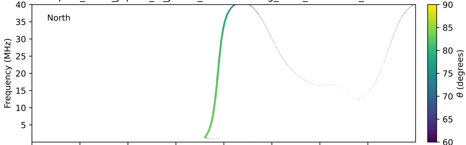
expres_earth_jupiter_io_jrm33_lossc-wid1deg_3kev_20031130_v11.cdf
