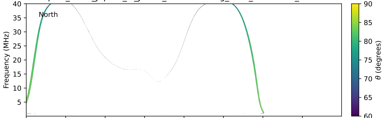
expres_earth_jupiter_io_jrm33_lossc-wid1deg_3kev_20031111_v11.cdf
