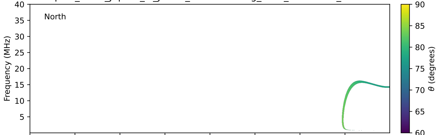
expres_earth_jupiter_io_jrm09_lossc-wid1deg_3kev_20031126_v11.cdf
