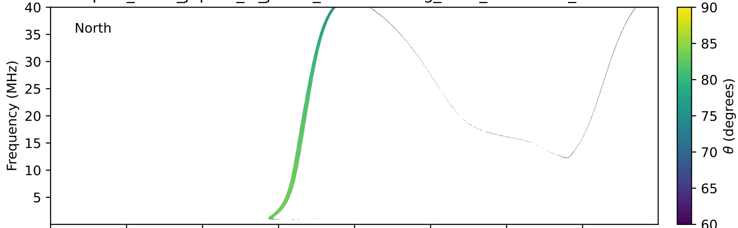
expres_earth_jupiter_io_jrm09_lossc-wid1deg_3kev_20031123_v11.cdf
