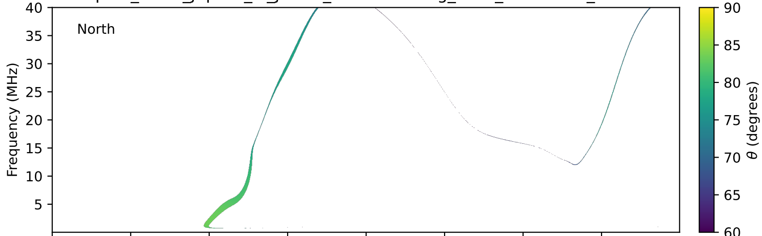
expres_earth_jupiter_io_jrm09_lossc-wid1deg_3kev_20031116_v11.cdf
