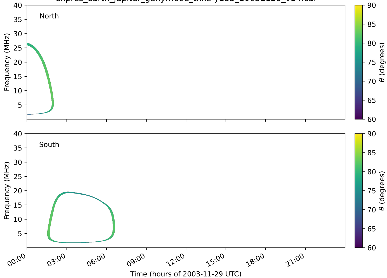
expres_earth_jupiter_ganymede_txka-y235_20031129_v14.cdf
