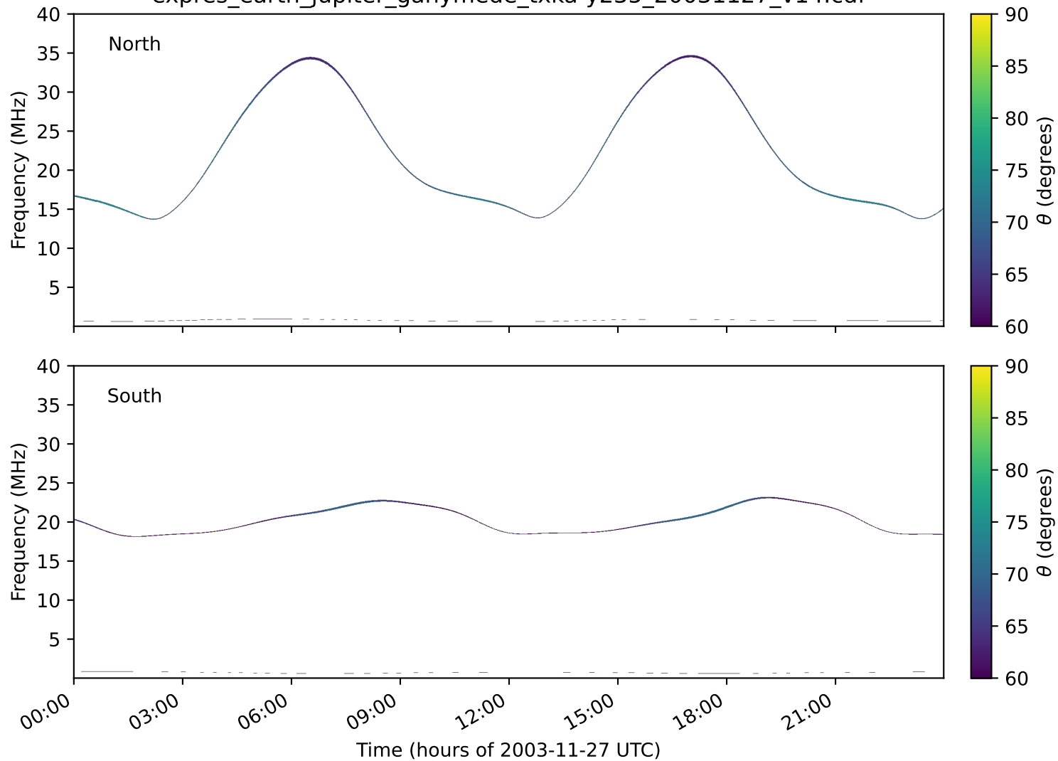
expres_earth_jupiter_ganymede_txka-y235_20031127_v14.cdf
