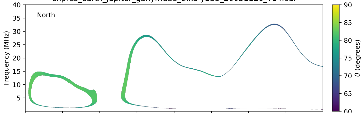
expres_earth_jupiter_ganymede_txka-y235_20031126_v14.cdf
