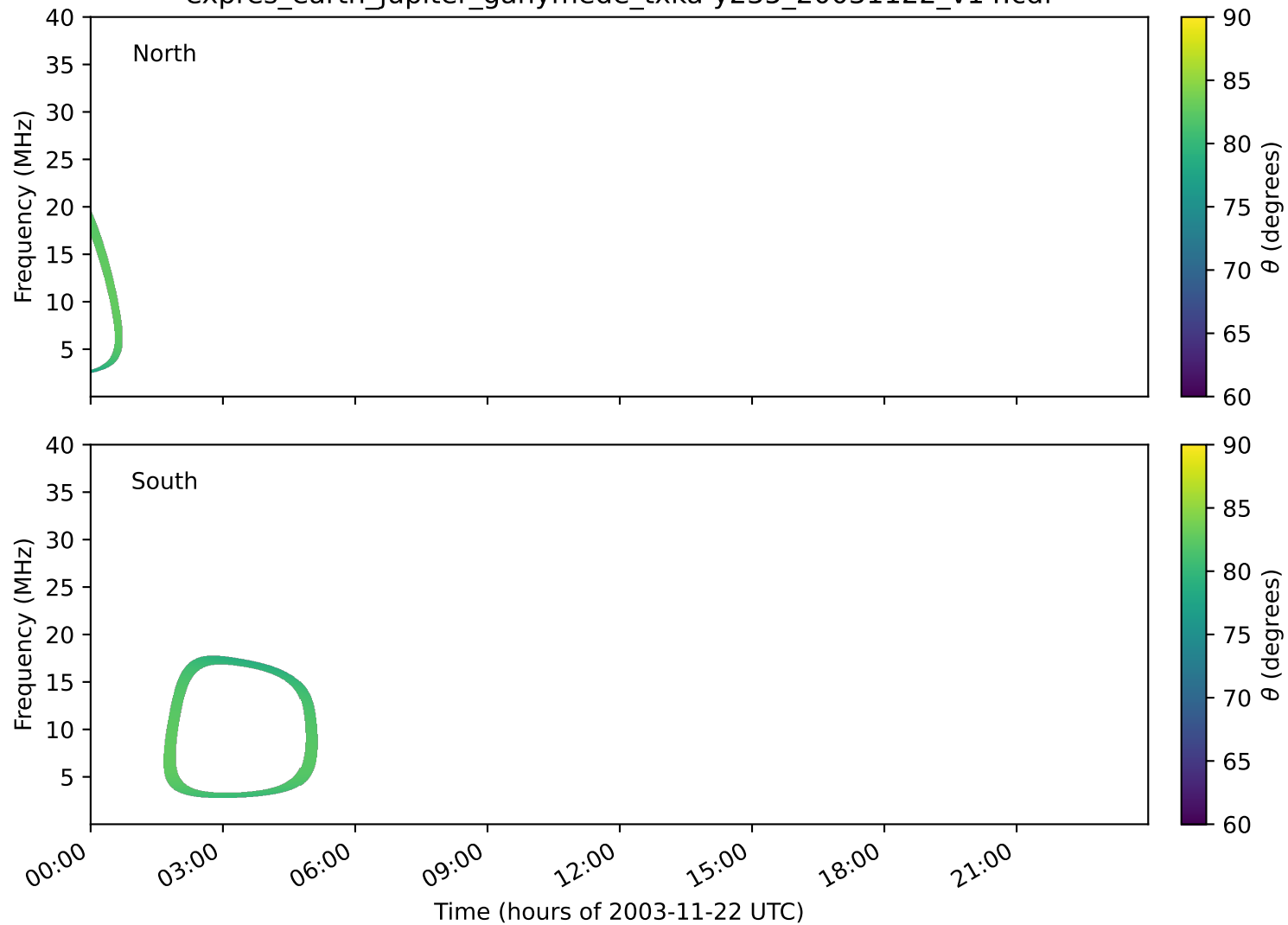
expres_earth_jupiter_ganymede_txka-y235_20031122_v14.cdf
