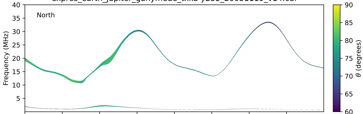
expres_earth_jupiter_ganymede_txka-y235_20031119_v14.cdf
