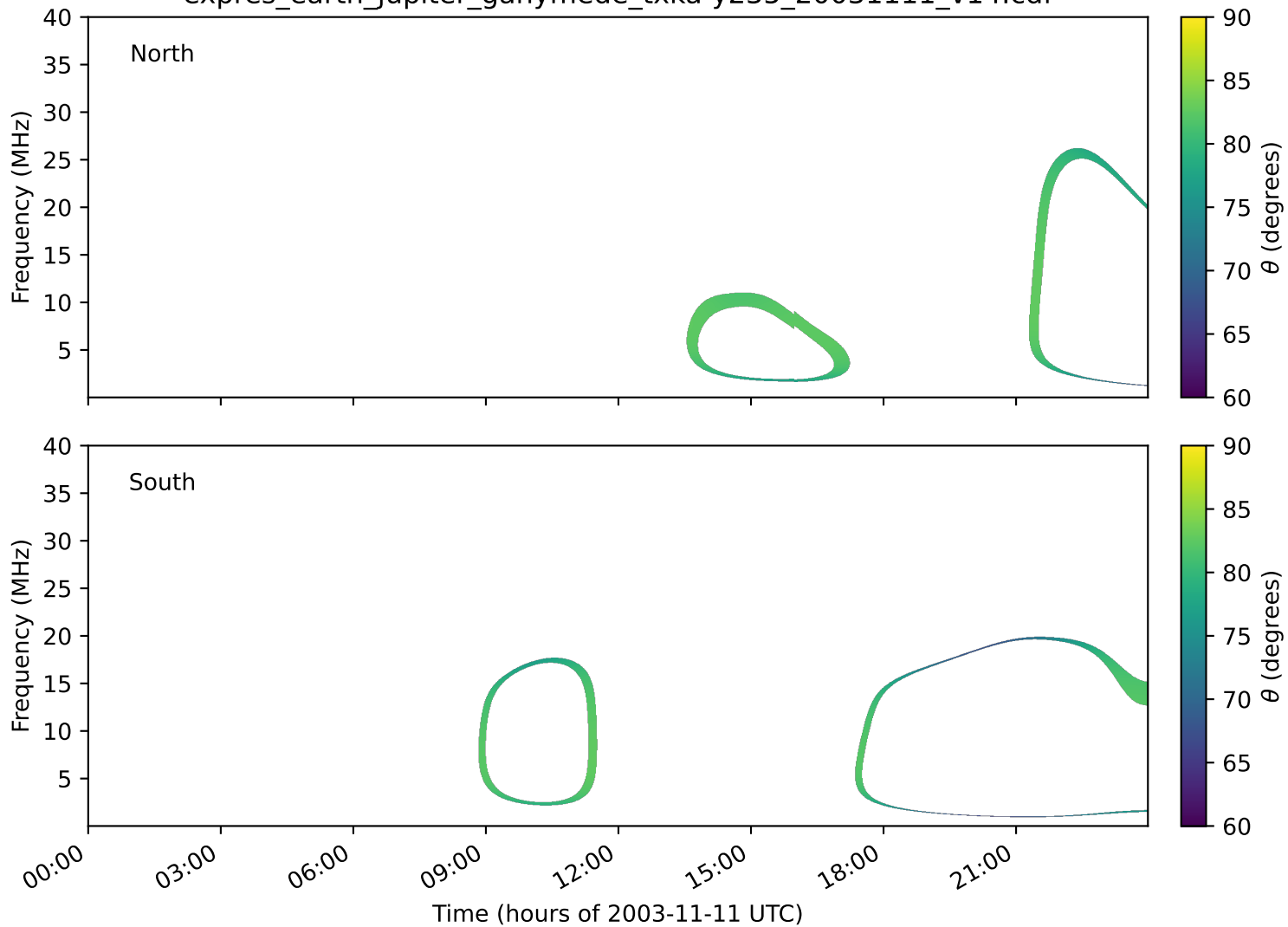
expres_earth_jupiter_ganymede_txka-y235_20031111_v14.cdf
