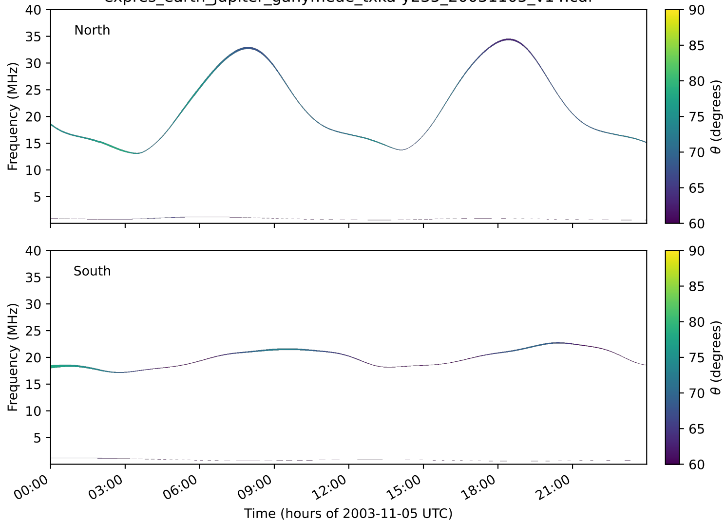
expres_earth_jupiter_ganymede_txka-y235_20031105_v14.cdf
