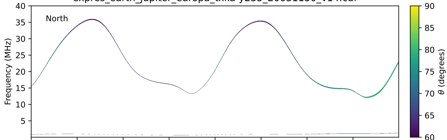
expres_earth_jupiter_europa_txka-y235_20031130_v14.cdf
