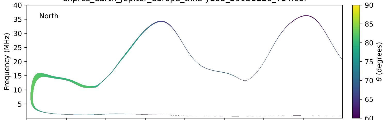
expres_earth_jupiter_europa_txka-y235_20031126_v14.cdf
