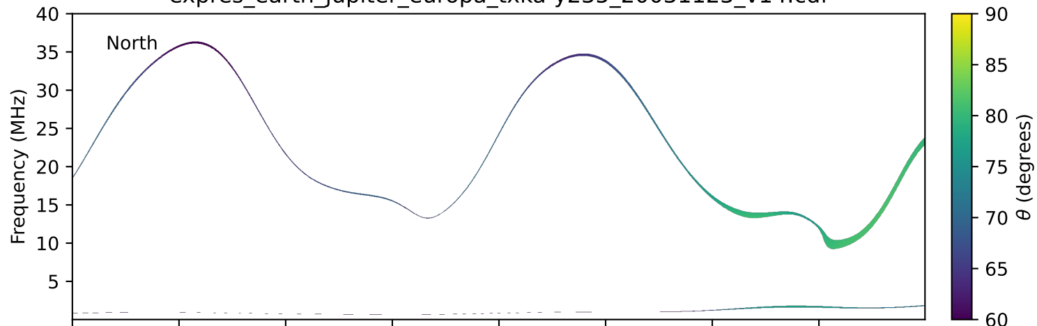
expres_earth_jupiter_europa_txka-y235_20031123_v14.cdf
