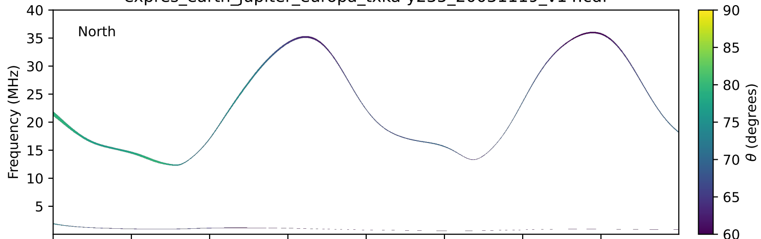
expres_earth_jupiter_europa_txka-y235_20031119_v14.cdf
