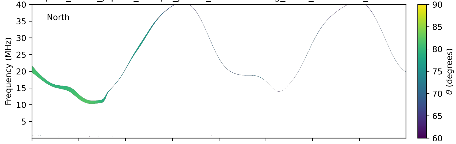
expres_earth_jupiter_europa_jrm33_lossc-wid1deg_3kev_20031119_v11.cdf
