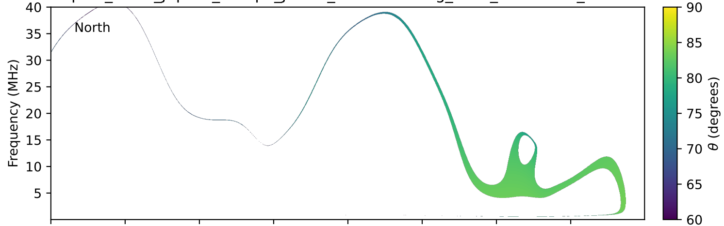
expres_earth_jupiter_europa_jrm33_lossc-wid1deg_3kev_20031109_v11.cdf
