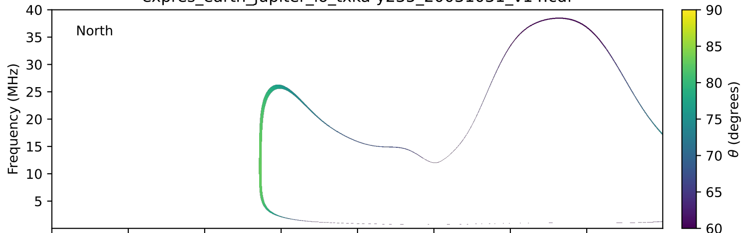
expres_earth_jupiter_io_txka-y235_20031031_v14.cdf
