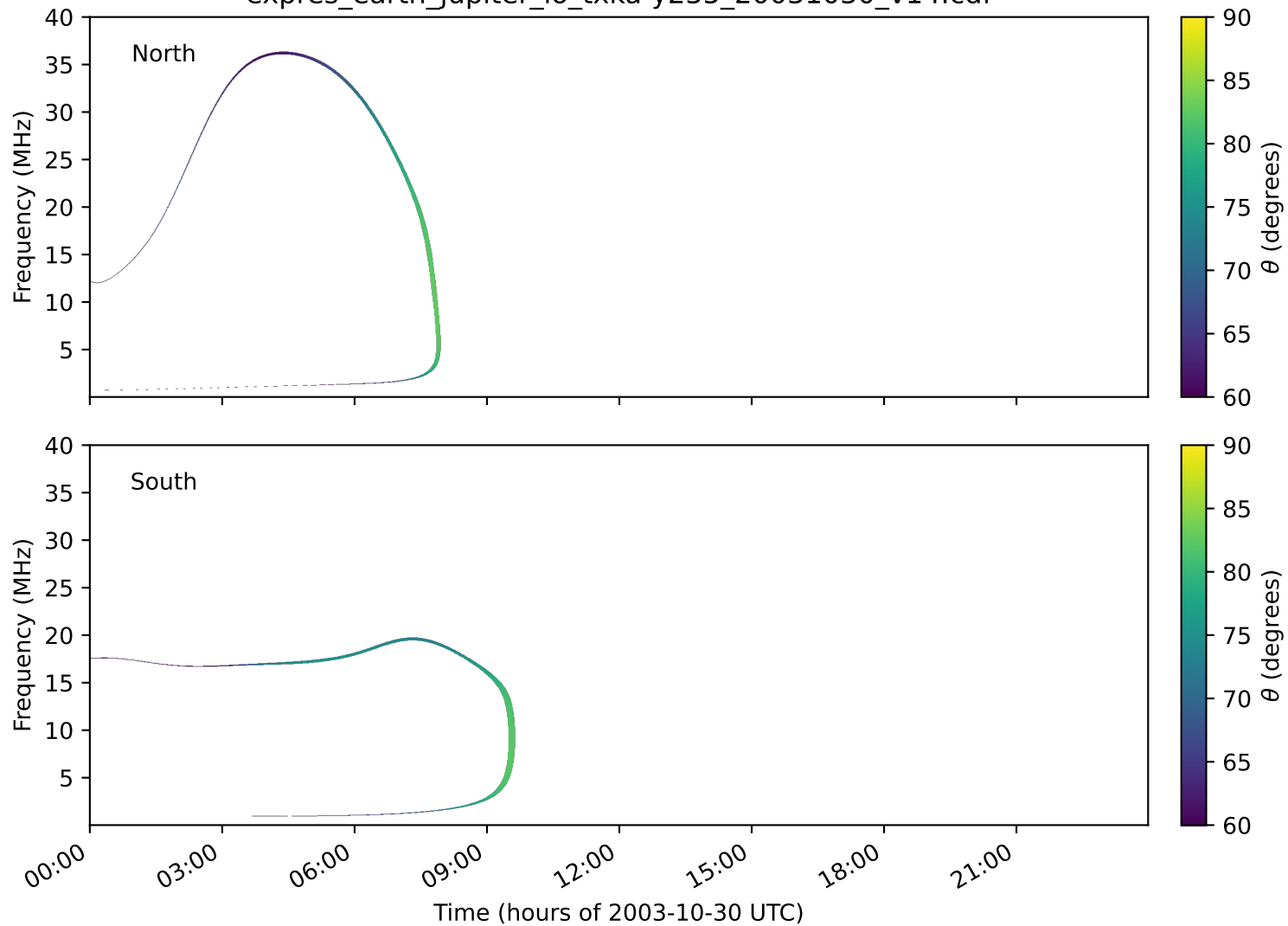
expres_earth_jupiter_io_txka-y235_20031030_v14.cdf
